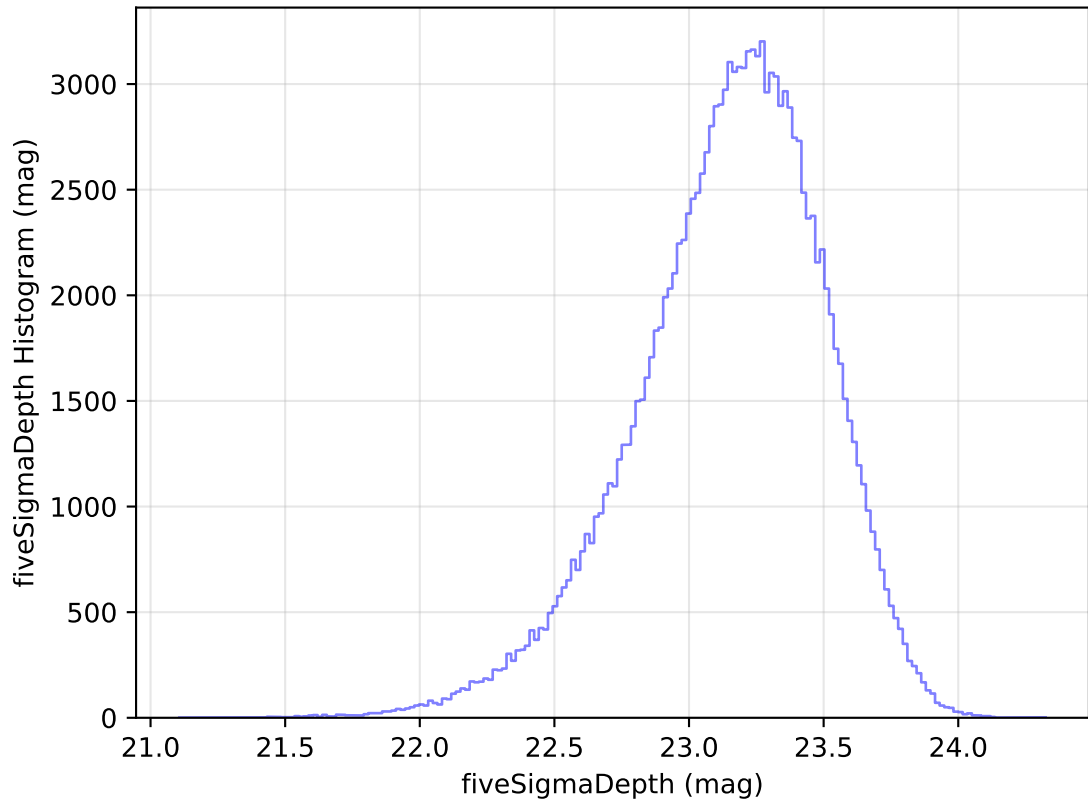
internal_u_expt30_nscale1.2v3.4_10yrs All sky u band: fiveSigmaDepth Histogram
