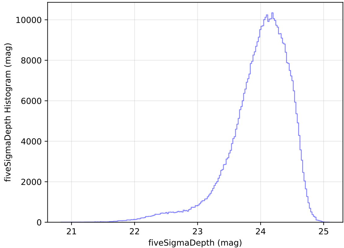
internal_u_expt30_nscale1.2v3.4_10yrs All sky r band: fiveSigmaDepth Histogram
