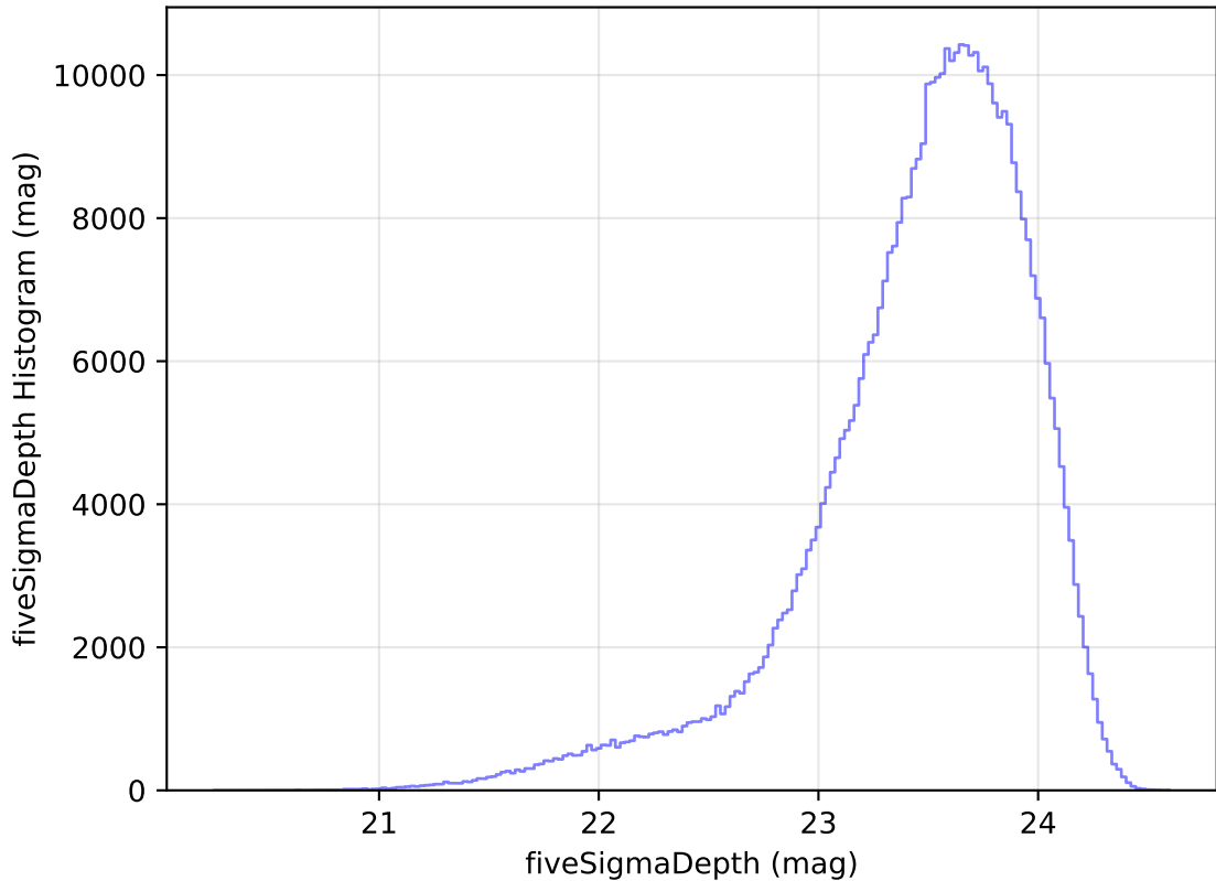
internal_u_expt30_nscale1.2v3.4_10yrs All sky i band: fiveSigmaDepth Histogram
