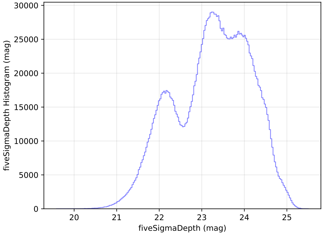
internal_u_expt30_nscale1.2v3.4_10yrs All sky all bands: fiveSigmaDepth Histogram
