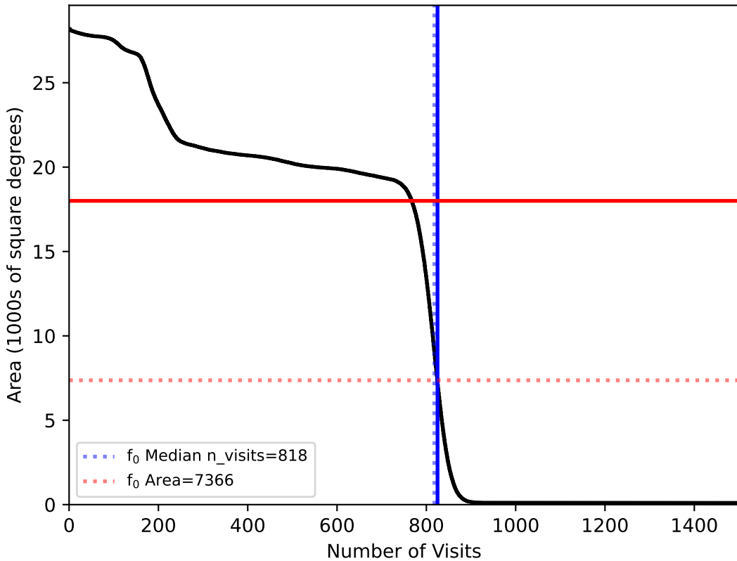
internal_u_expt30_nscale1.2v3.4_10yrs All sky: f0
