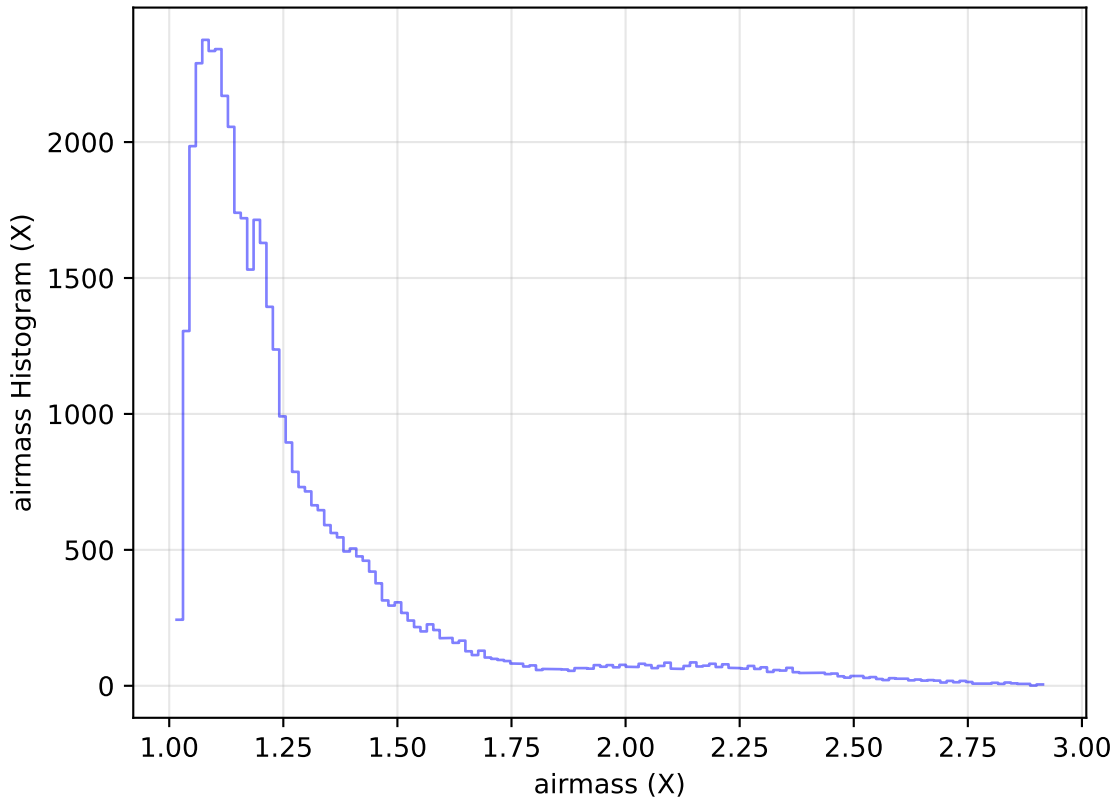
internal_u_expt30_nscale1.2v3.4_10yrs Yr 1 z band: airmass Histogram
