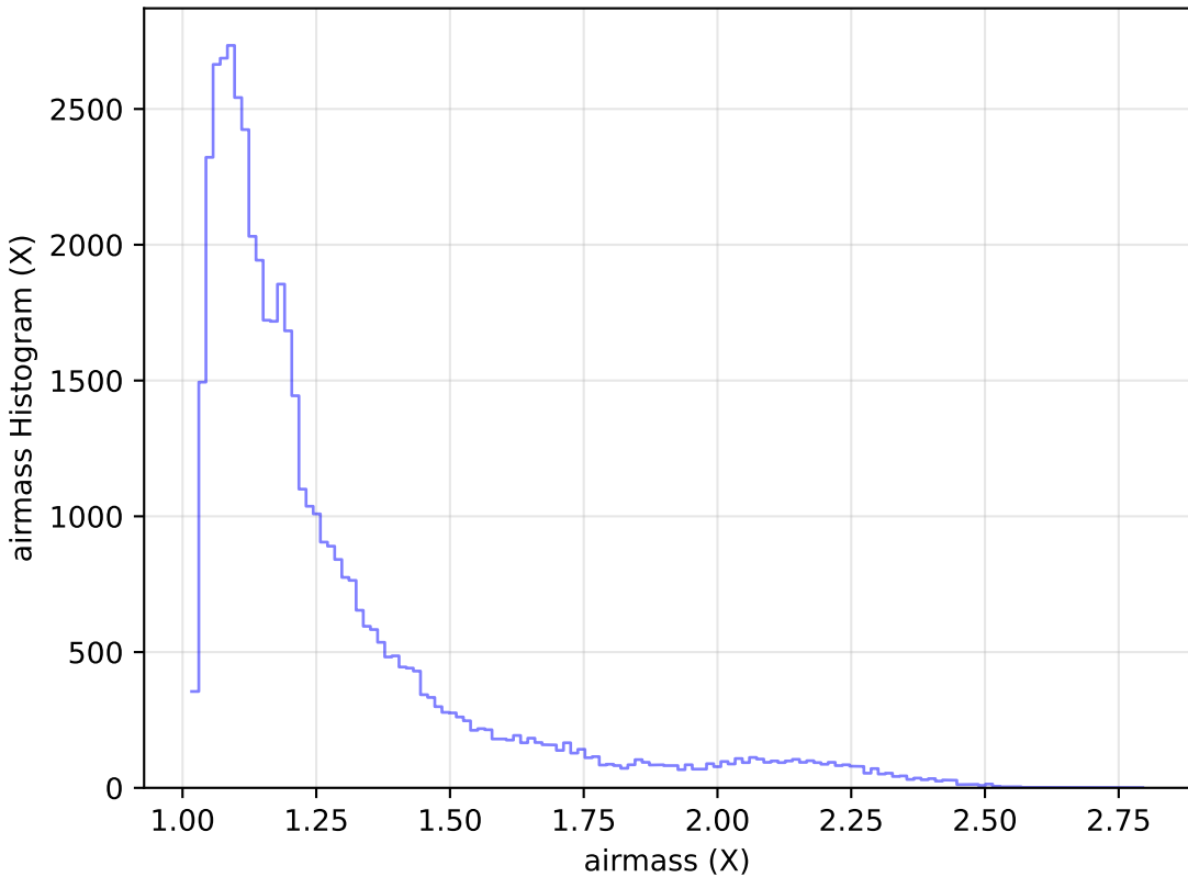
internal_u_expt30_nscale1.2v3.4_10yrs Yr 1 r band: airmass Histogram
