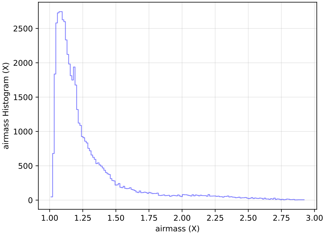
internal_u_expt30_nscale1.2v3.4_10yrs Yr 1 i band: airmass Histogram
