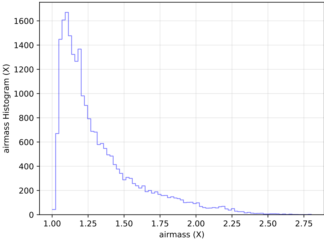
internal_u_expt30_nscale1.2v3.4_10yrs Yr 1 g band: airmass Histogram
