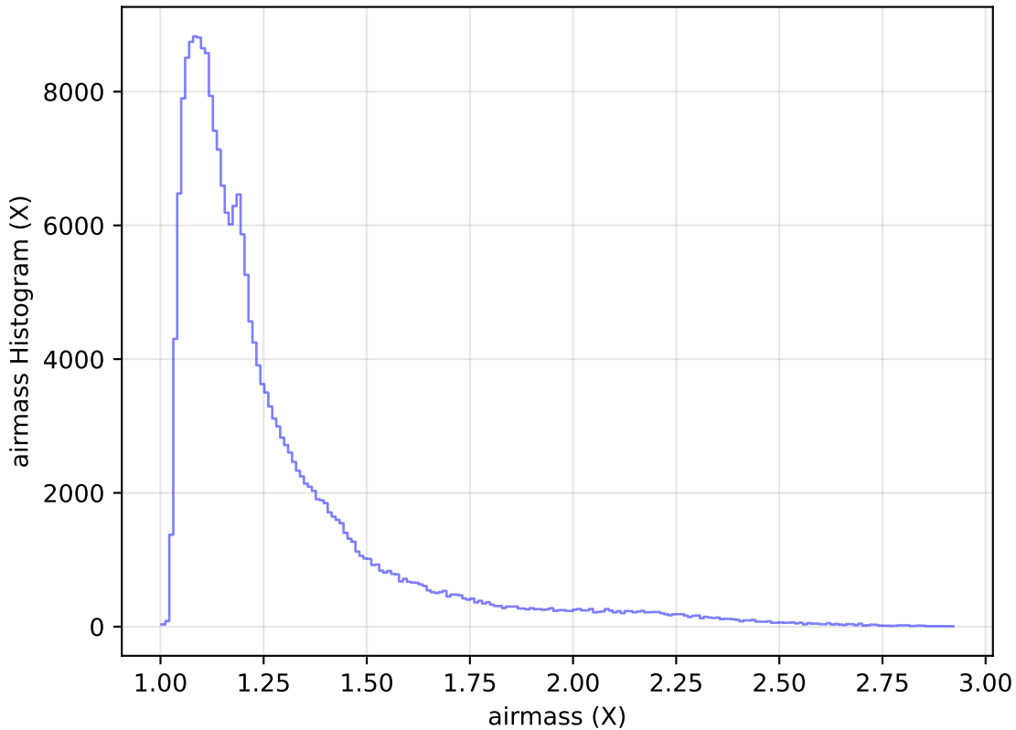
internal_u_expt30_nscale1.2v3.4_10yrs Yr 1 all bands: airmass Histogram
