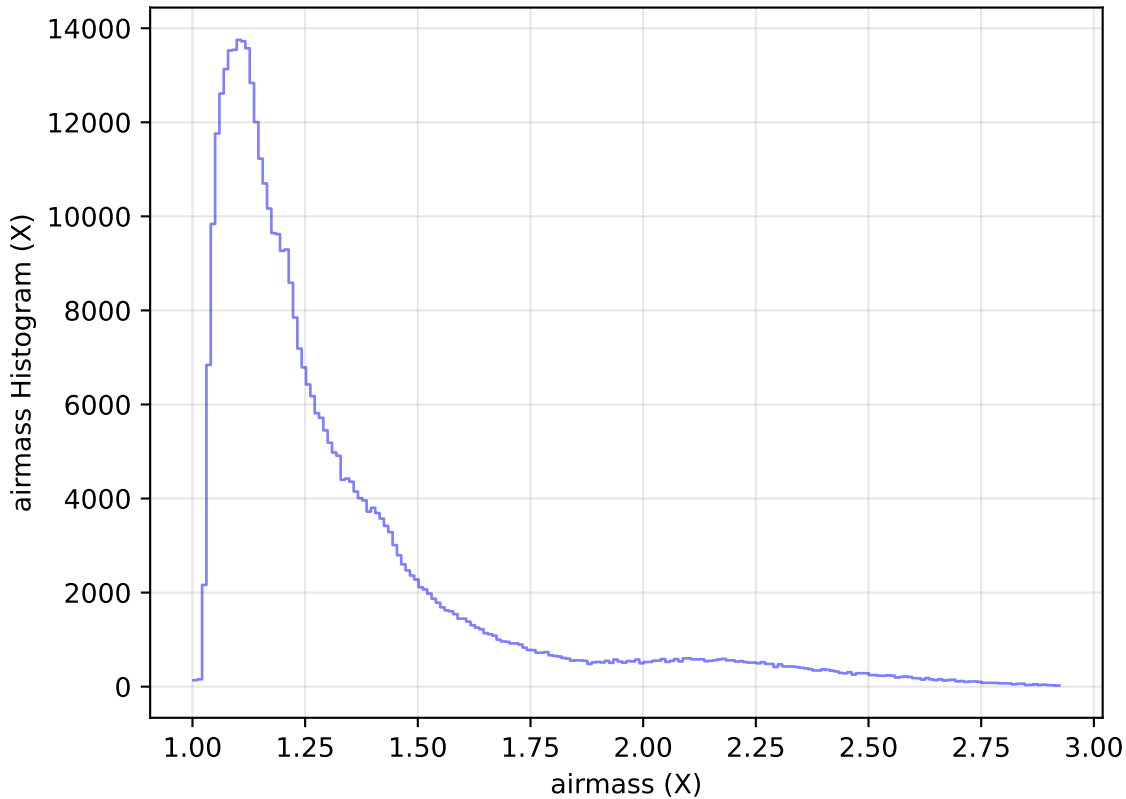
internal_u_expt30_nscale1.2v3.4_10yrs WFD z band: airmass Histogram
