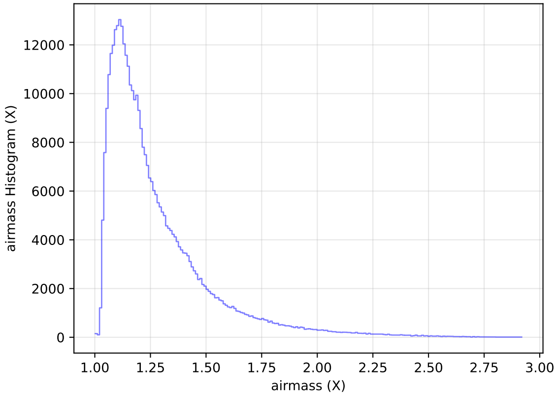
internal_u_expt30_nscale1.2v3.4_10yrs WFD y band: airmass Histogram
