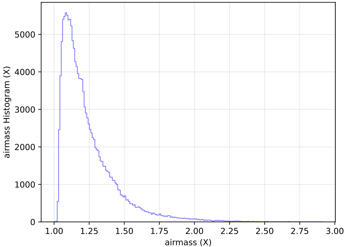
internal_u_expt30_nscale1.2v3.4_10yrs WFD u band: airmass Histogram
