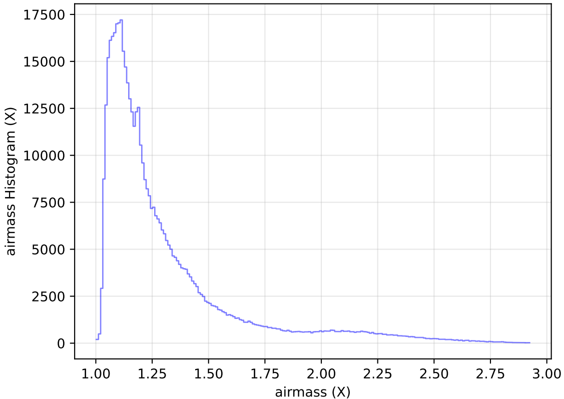
internal_u_expt30_nscale1.2v3.4_10yrs WFD i band: airmass Histogram
