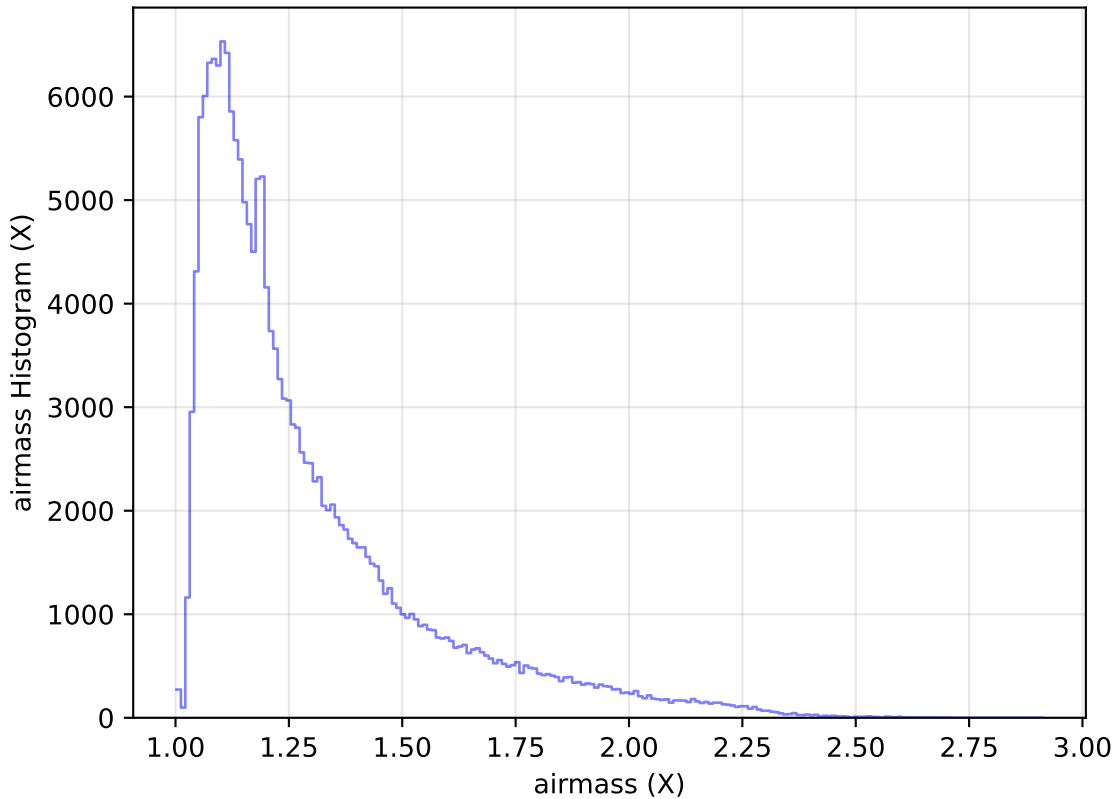
internal_u_expt30_nscale1.2v3.4_10yrs WFD g band: airmass Histogram
