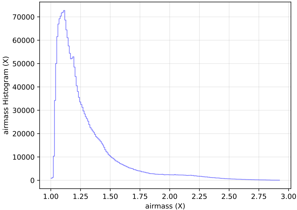
internal_u_expt30_nscale1.2v3.4_10yrs WFD all bands: airmass Histogram
