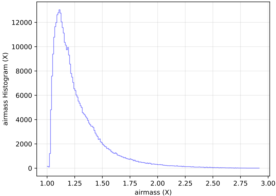
internal_u_expt30_nscale1.2v3.4_10yrs All sky y band: airmass Histogram
