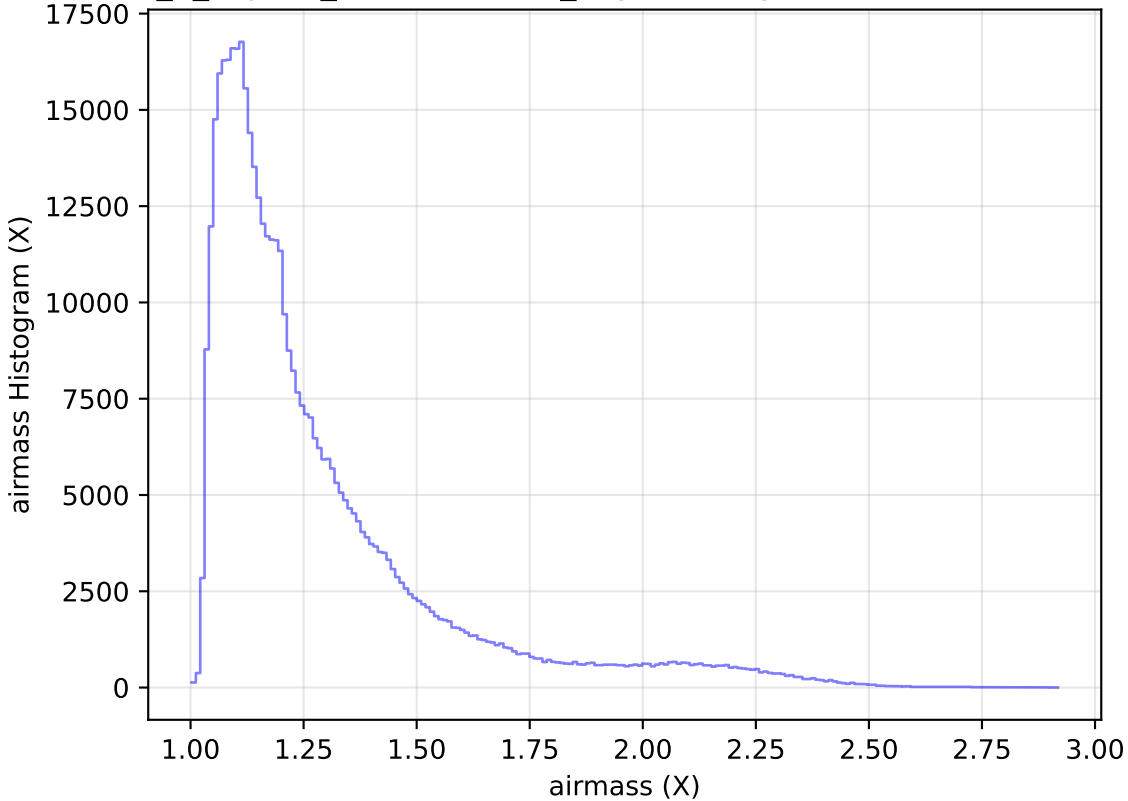
internal_u_expt30_nscale1.2v3.4_10yrs All sky r band: airmass Histogram
