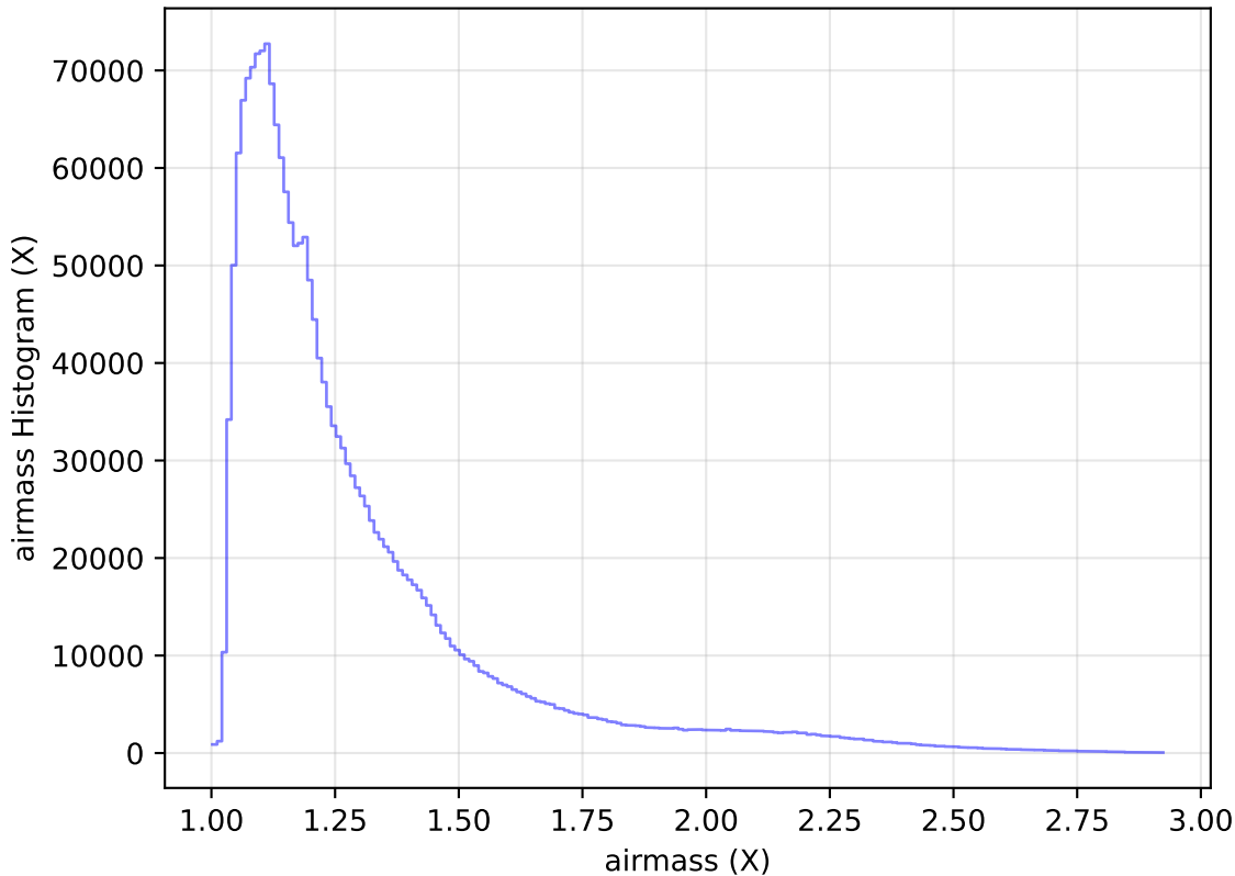
internal_u_expt30_nscale1.2v3.4_10yrs All sky all bands: airmass Histogram
