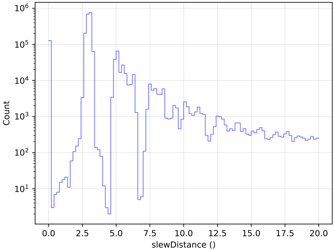
internal_u_expt30_nscale1.2v3.4_10yrs All visits: Zoom Slew Distance Histogram
