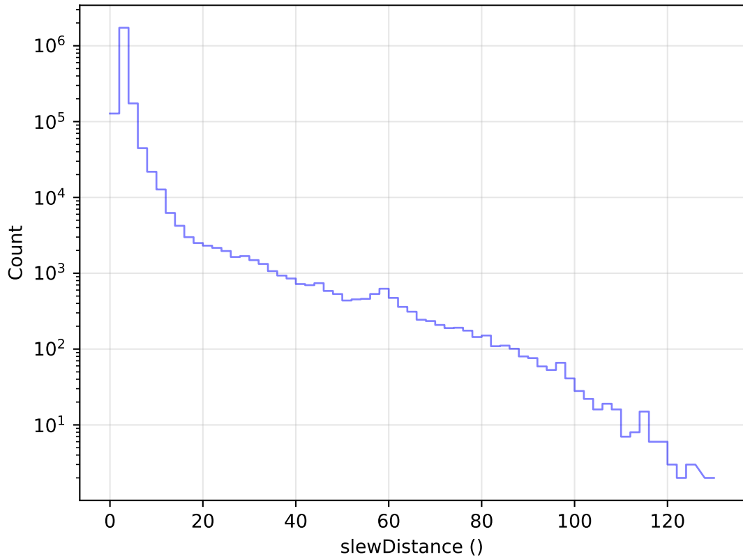
internal_u_expt30_nscale1.2v3.4_10yrs All visits: Slew Distance Histogram
