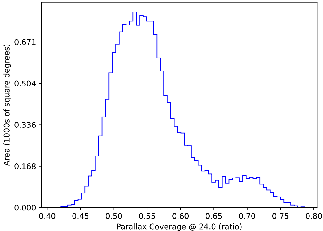
internal_u_expt30_nscale1.2v3.4_10yrs WFD: Parallax Coverage @ 24.0
