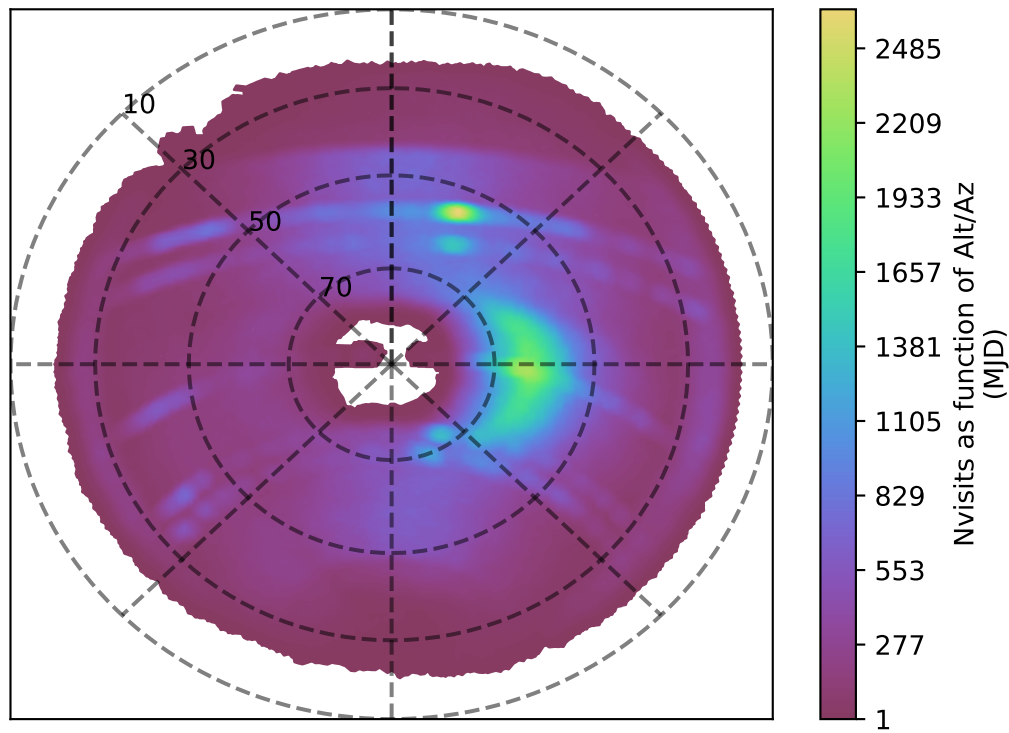
internal_u_expt30_nscale1.2v3.4_10yrs z band: Nvisits as function of Alt/Az
