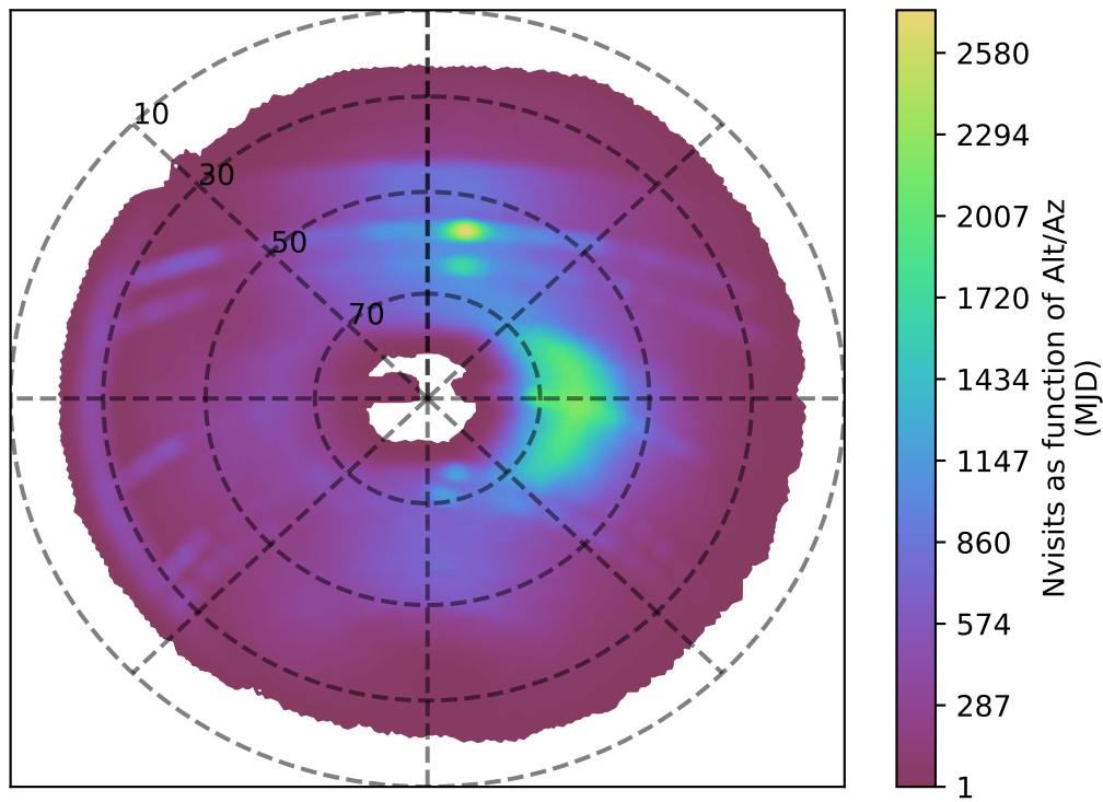
internal_u_expt30_nscale1.2v3.4_10yrs r band: Nvisits as function of Alt/Az
