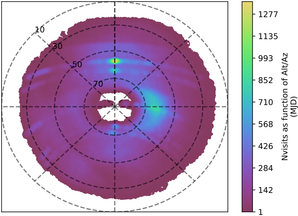
internal_u_expt30_nscale1.2v3.4_10yrs g band: Nvisits as function of Alt/Az
