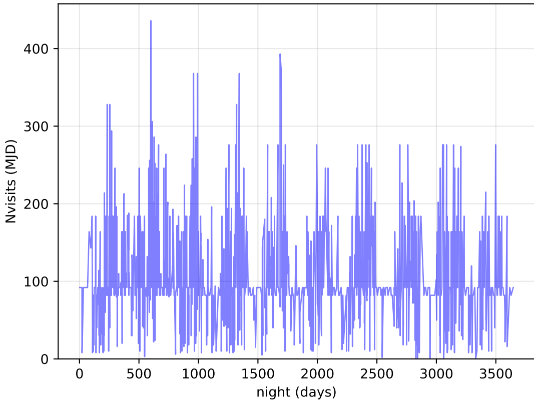
internal_u_expt30_nscale1.2v3.4_10yrs DDF: Nvisits
