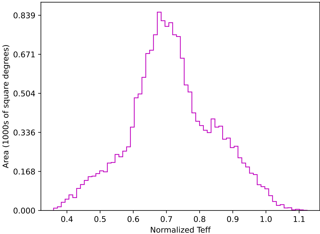
internal_u_expt30_nscale1.2v3.4_10yrs WFD z band: Normalized Teff
