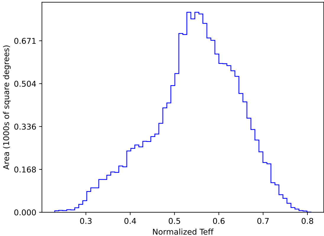
internal_u_expt30_nscale1.2v3.4_10yrs WFD y band: Normalized Teff
