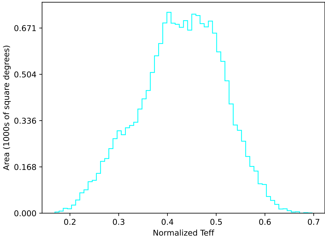
internal_u_expt30_nscale1.2v3.4_10yrs WFD u band: Normalized Teff
