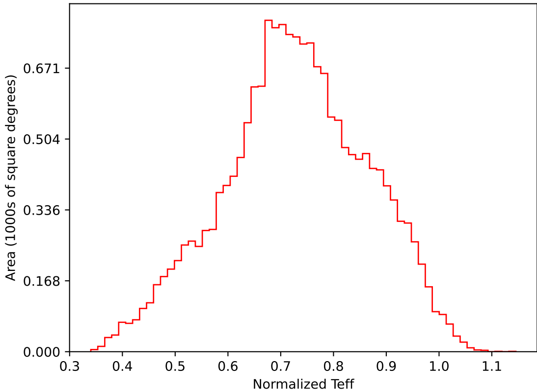
internal_u_expt30_nscale1.2v3.4_10yrs WFD i band: Normalized Teff
