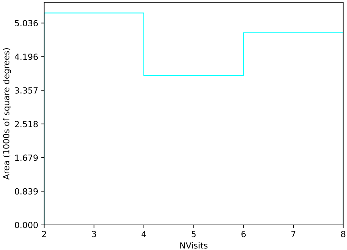
internal_u_expt30_nscale1.2v3.4_10yrs Yr 3-4 u band: NVisits
