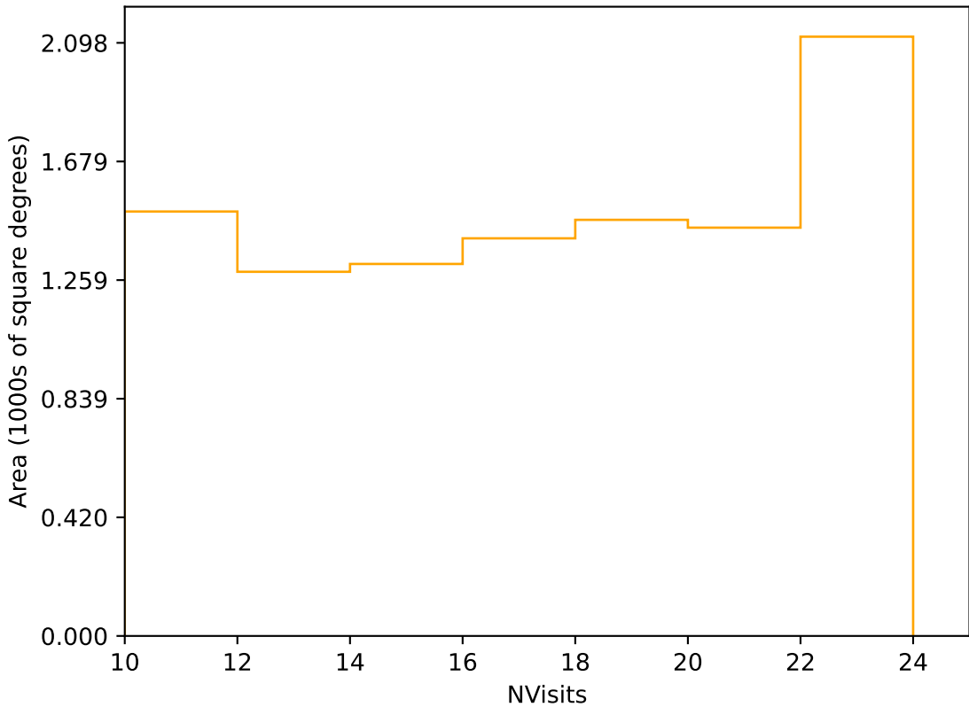
internal_u_expt30_nscale1.2v3.4_10yrs Yr 3-4 r band: NVisits
