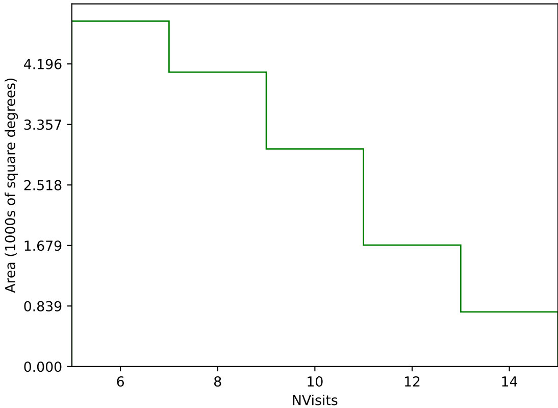
internal_u_expt30_nscale1.2v3.4_10yrs Yr 3-4 g band: NVisits
