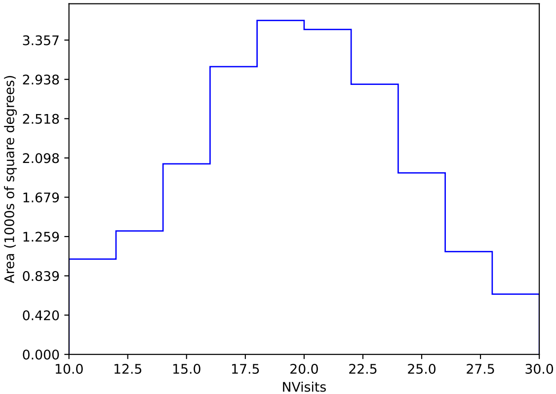
internal_u_expt30_nscale1.2v3.4_10yrs Yr 1 y band: NVisits
