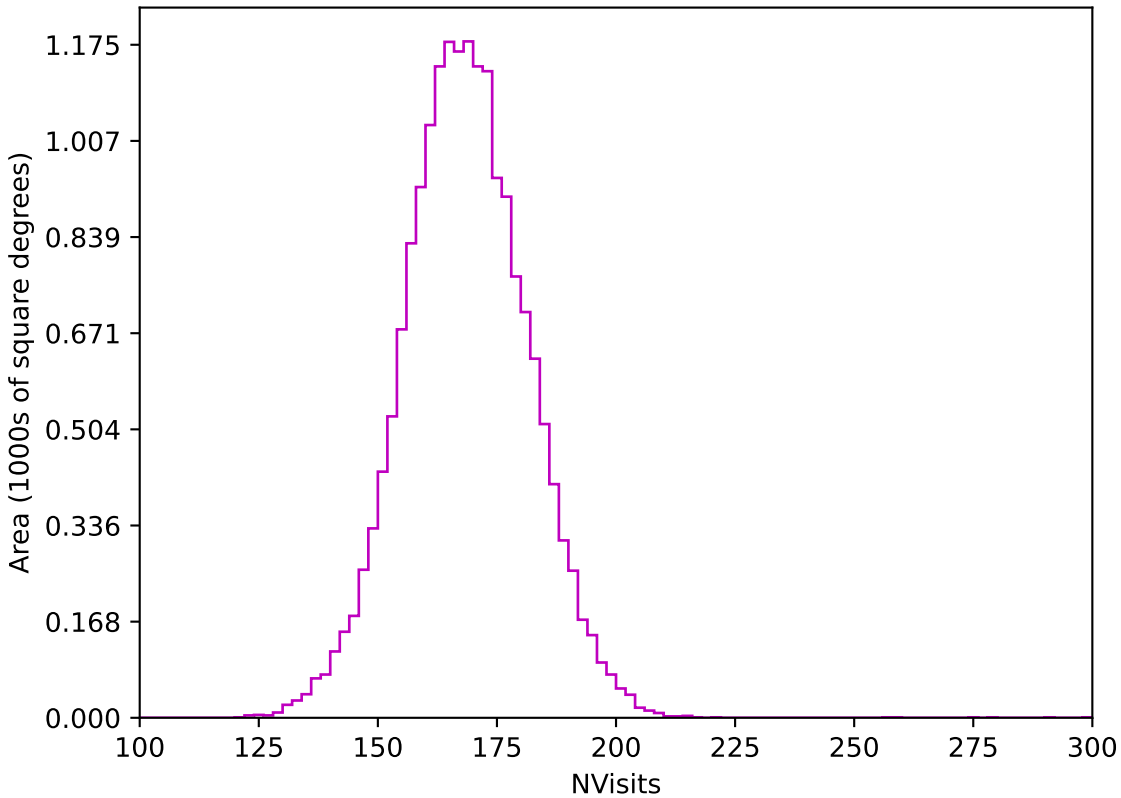
internal_u_expt30_nscale1.2v3.4_10yrs WFD z band: NVisits
