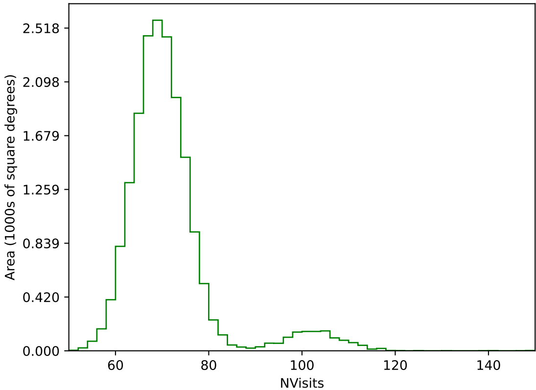
internal_u_expt30_nscale1.2v3.4_10yrs WFD g band: NVisits
