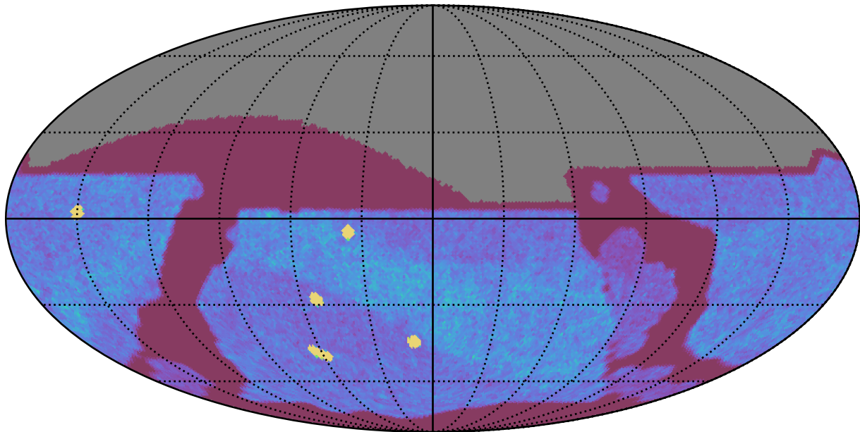
internal_u_expt30_nscale1.2v3.4_10yrs All sky z band: NVisits
