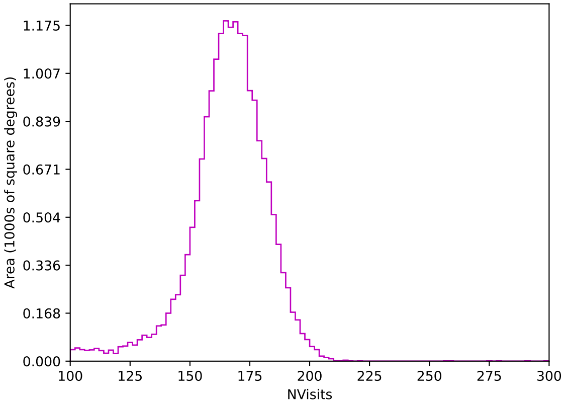
internal_u_expt30_nscale1.2v3.4_10yrs All sky z band: NVisits
