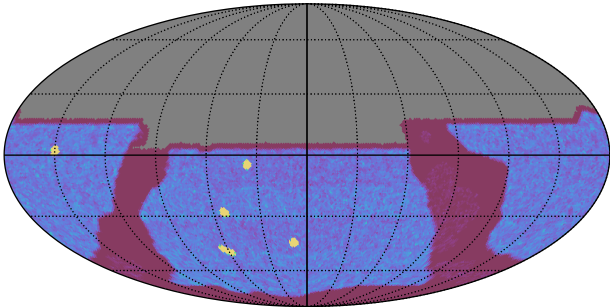
internal_u_expt30_nscale1.2v3.4_10yrs All sky y band: NVisits
