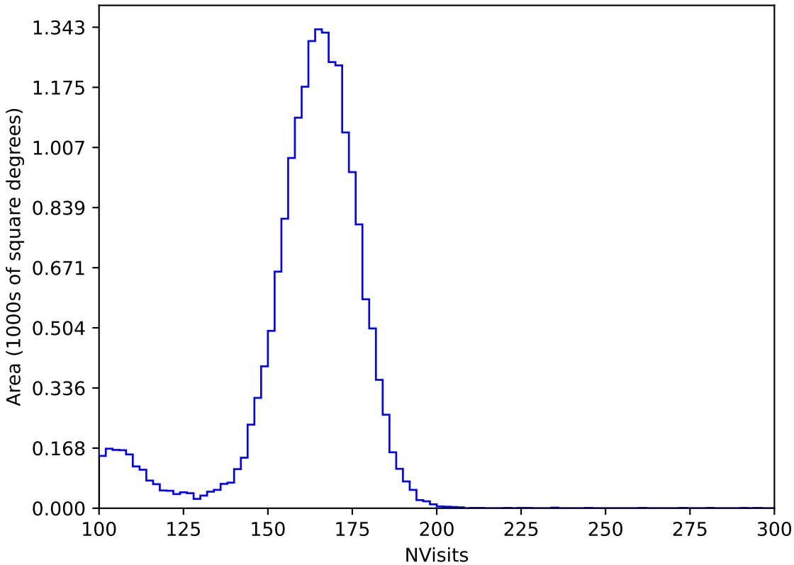
internal_u_expt30_nscale1.2v3.4_10yrs All sky y band: NVisits
