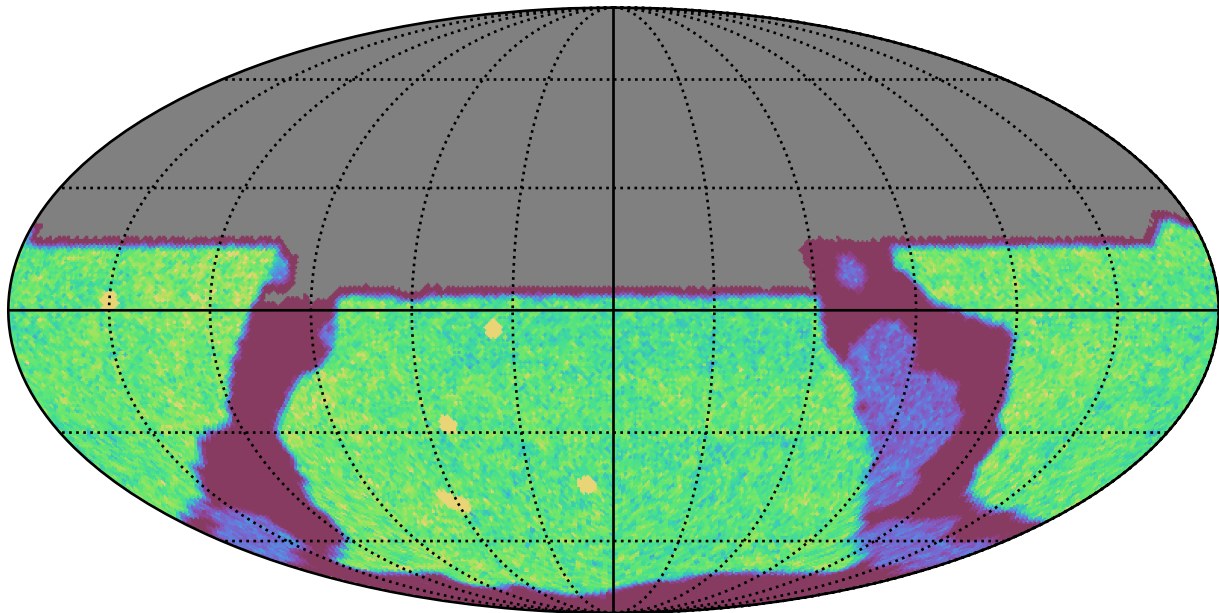
internal_u_expt30_nscale1.2v3.4_10yrs All sky u band: NVisits
