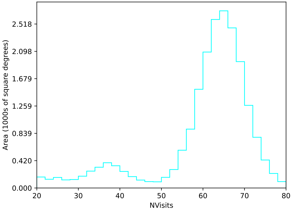
internal_u_expt30_nscale1.2v3.4_10yrs All sky u band: NVisits
