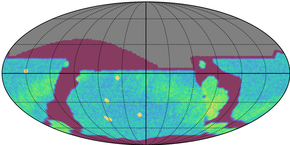
internal_u_expt30_nscale1.2v3.4_10yrs All sky r band: NVisits
