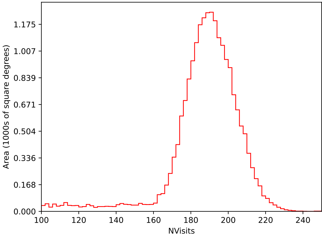
internal_u_expt30_nscale1.2v3.4_10yrs All sky i band: NVisits
