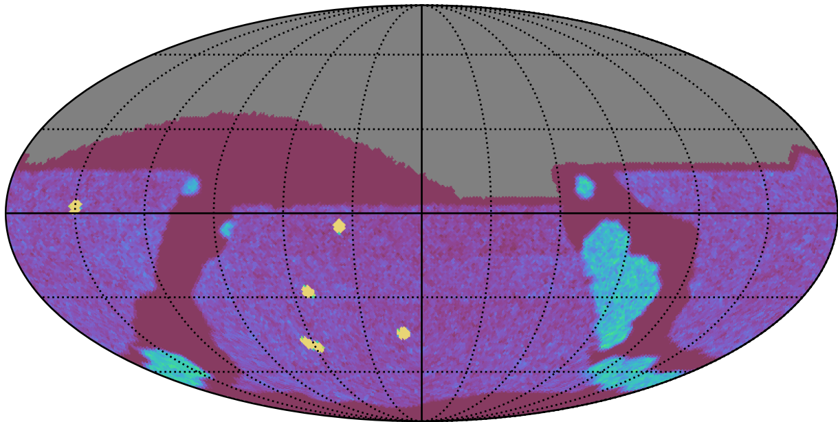
internal_u_expt30_nscale1.2v3.4_10yrs All sky g band: NVisits
