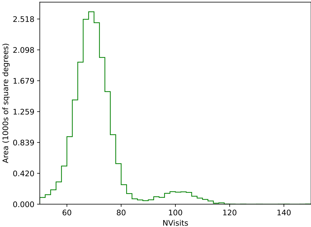
internal_u_expt30_nscale1.2v3.4_10yrs All sky g band: NVisits
