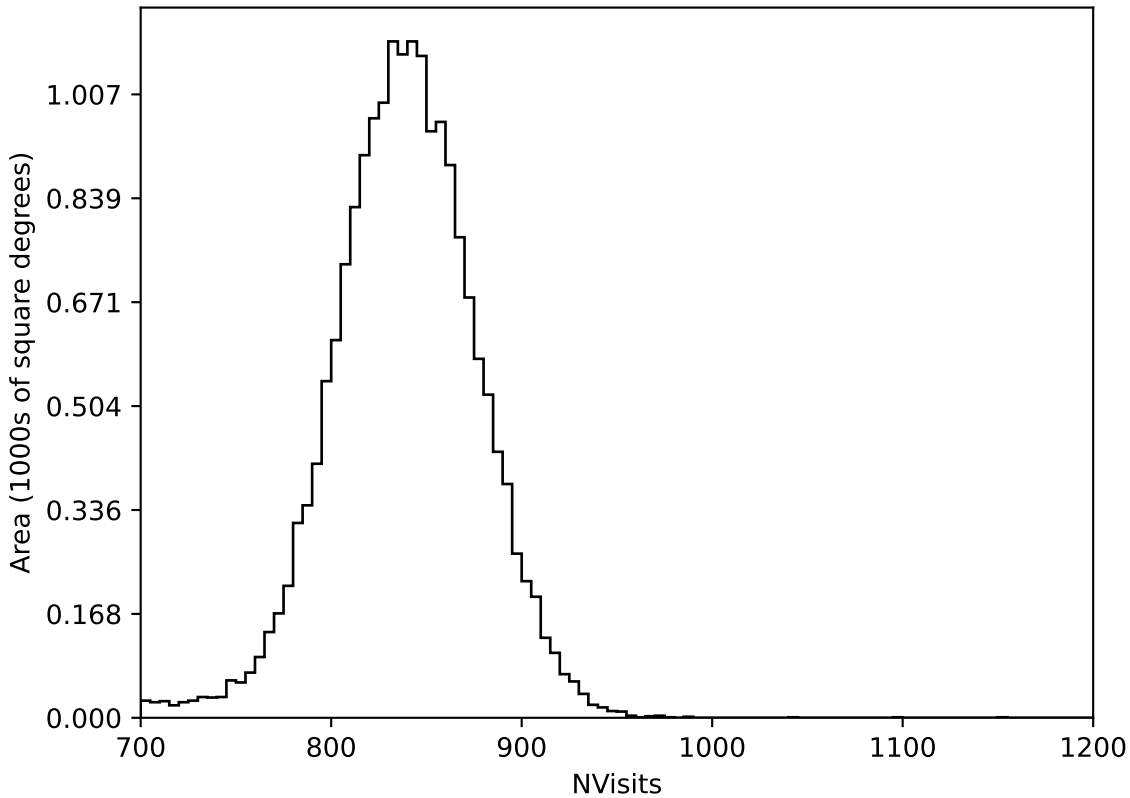
internal_u_expt30_nscale1.2v3.4_10yrs All sky all bands: NVisits
