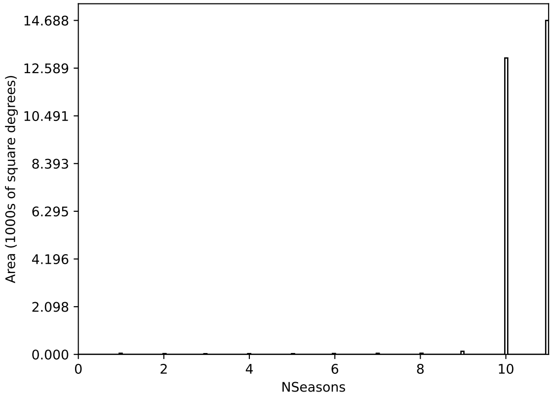
internal_u_expt30_nscale1.2v3.4_10yrs All sky all bands: NSeasons
