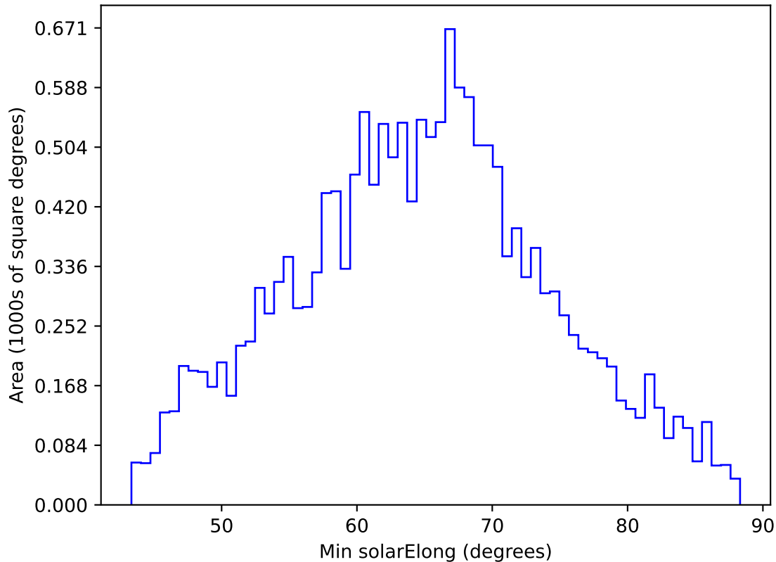
internal_u_expt30_nscale1.2v3.4_10yrs WFD y band: Min solarElong
