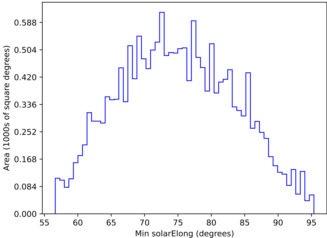
internal_u_expt30_nscale1.2v3.4_10yrs WFD u band: Min solarElong
